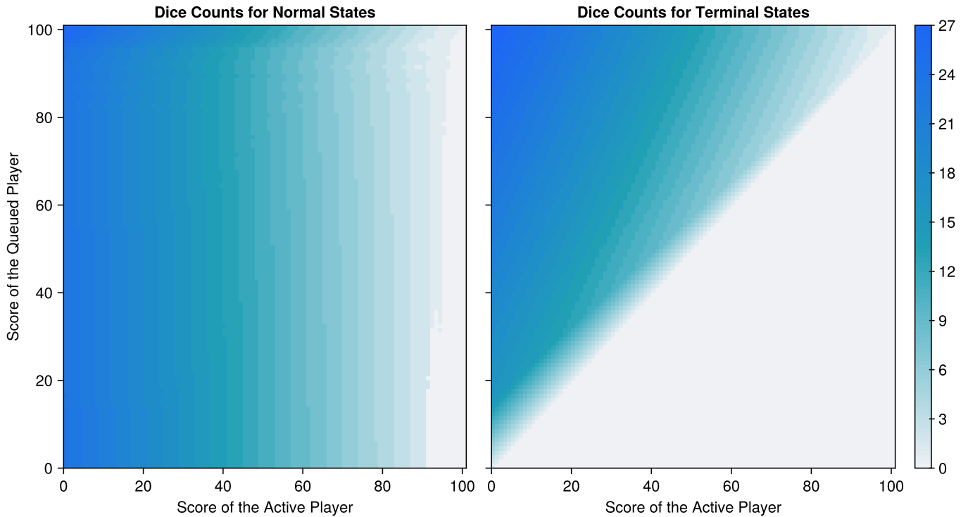
Figure 2 | Optimal rolls for each state given the standard ruleset of M = 100, s = 6 . For normal states, there is a weak correlation between the opponents score and the optimal number of dice to throw. For terminal states, the optimal policy while ahead is to stand . For terminal states where victory is not guaranteed, there is a positive correlation between the difference in the queued score and the active score, and the optimal number of dice to roll. This accounts for the diagonal bands.
